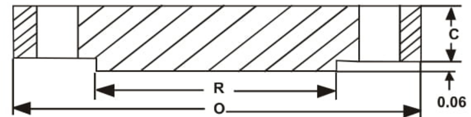
Blind
