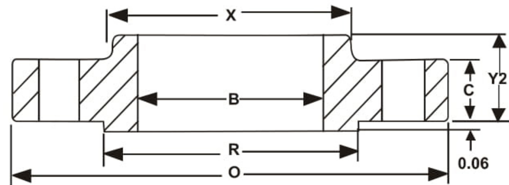
Slip On
