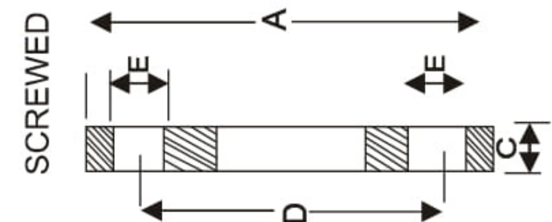
BS 10 Pipes
