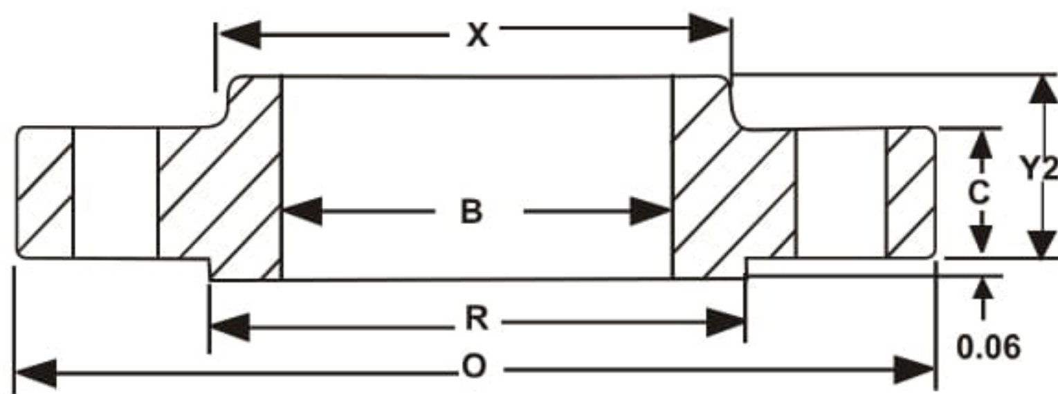
Slip On
