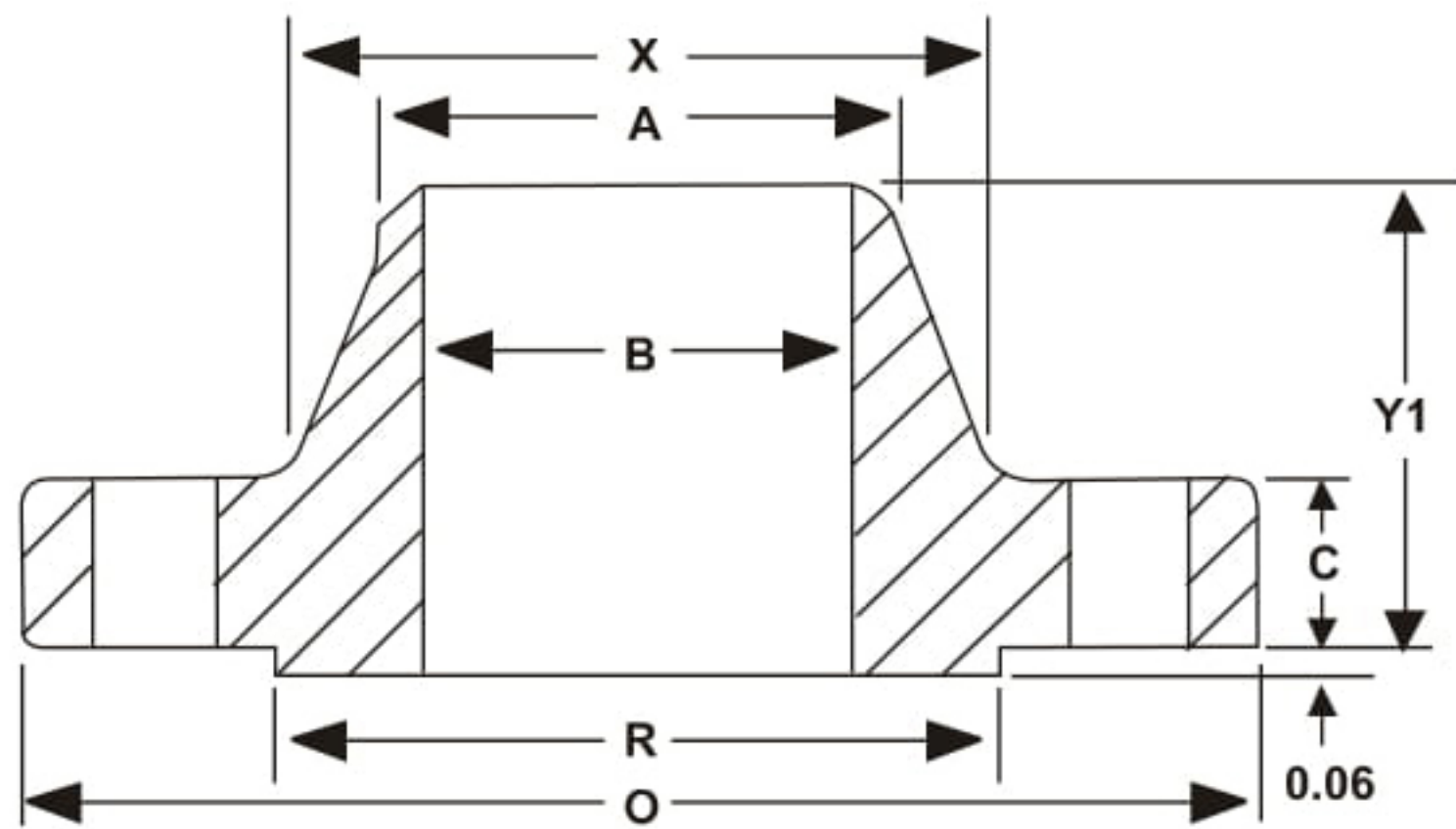
Weld Neck
