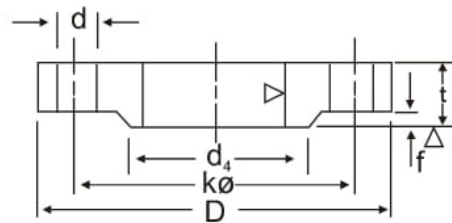
SLIP-ON
