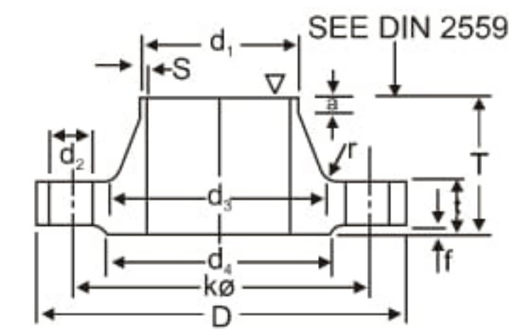
WELDING NECK
