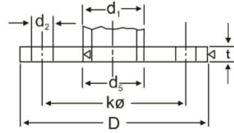
SLIP-ON
