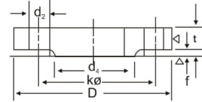
BLIND
