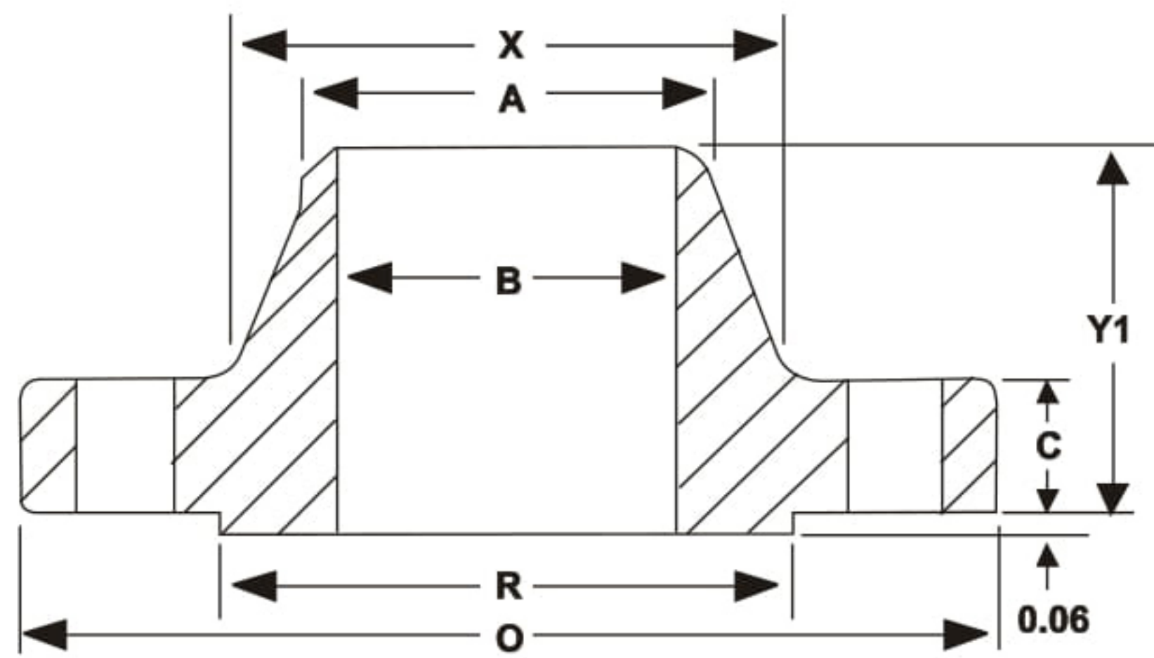
Weld Neck (B determined by Purchaser)
